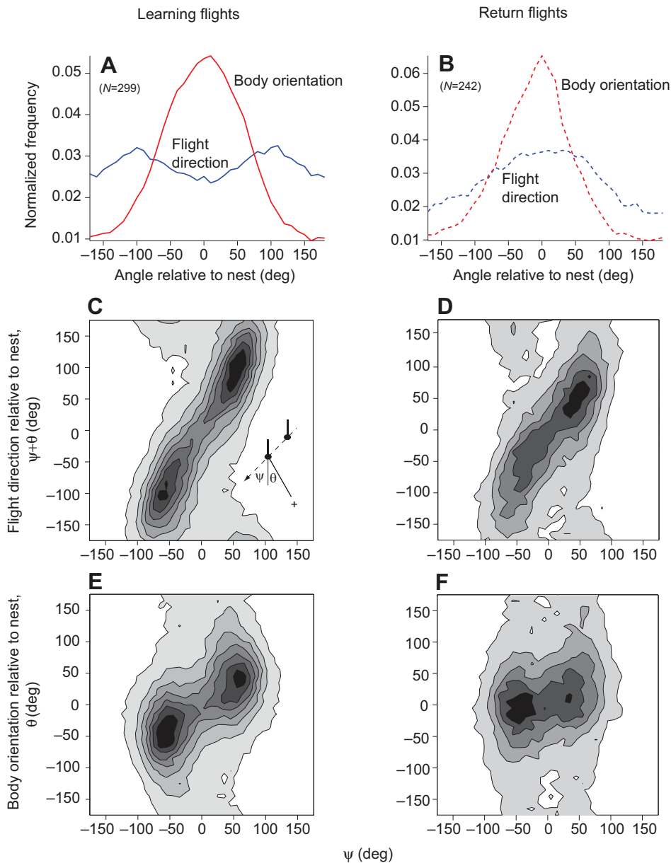
Fig. 1. The nest-directed nature of learning and return flights. (A,B) Frequency distributions of body orientations (red lines, \theta , see inset in C) and flight directions (blue lines, \psi+\theta ) relative to the nest are pooled over 299 learning (left-hand column) and 242 return (right-hand column) flights. The flights come from different groups of bees each with one or two cylinders near the nest. (C,D) Contour plot of flight direction relative to nest ( \psi+\theta ) versus \psi ; inset illustrates \psi , \theta and the nest (+). (E,F) Contour plot of body orientation ( \theta ) versus \psi . Contour plots in (C,E) comprise 169,798 data points and both plots step in multiples of 100 from white (<100) to black ( \geq 700 ). The plots of (D,F) comprise 64,015 data points and both plots step in multiples of 50 from white (<50) to black ( \geq 250 ). Here and in other figures angular values increase clockwise (see inset to E), frequency distributions are normalized so that their area is 1, and, unless specified otherwise, bin widths are 10 deg.
