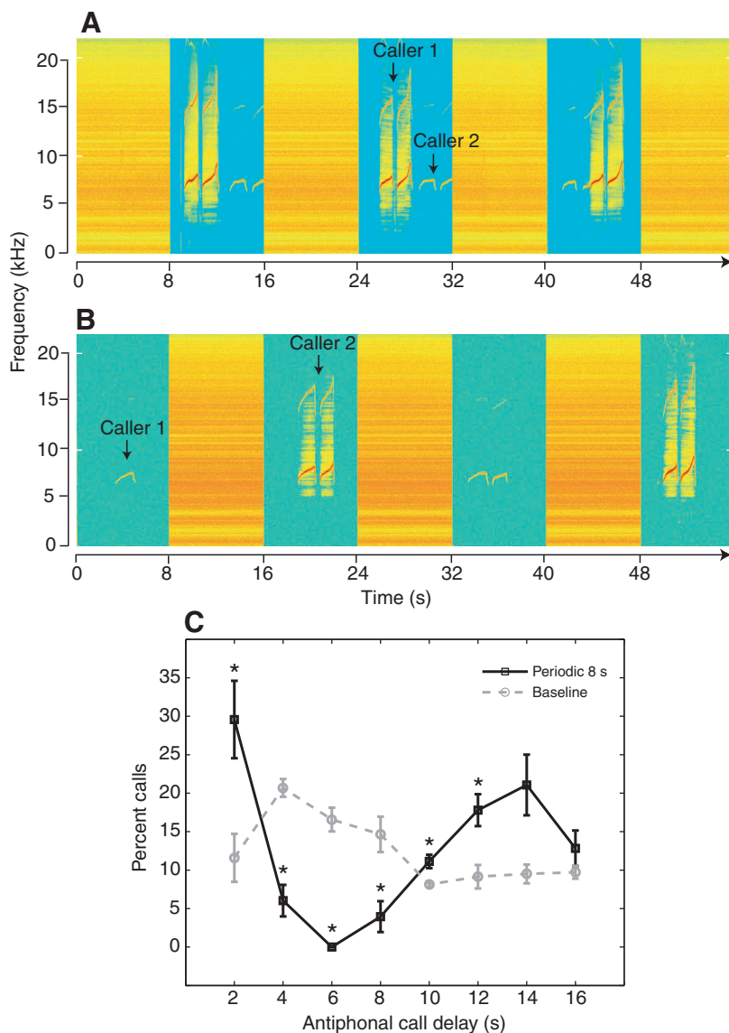
Fig. 4. Antiphonal calling in the presence of periodic noise. (A) Example of antiphonal call exchange between caller 1 and caller 2 within the same silent gaps in the periodic 8 s condition. (B) Example of antiphonal call exchange between consecutive silent gaps in the periodic 8 s condition. (C) Comparison of the periodic 8 s and baseline antiphonal call delays of all pairs in 2 s bins. Means \pm s.e.m. of percent calls are shown with statistically significant differences between periodic 8 s noise condition and baseline ( *P < 0.05 ) indicated by an asterisk.
