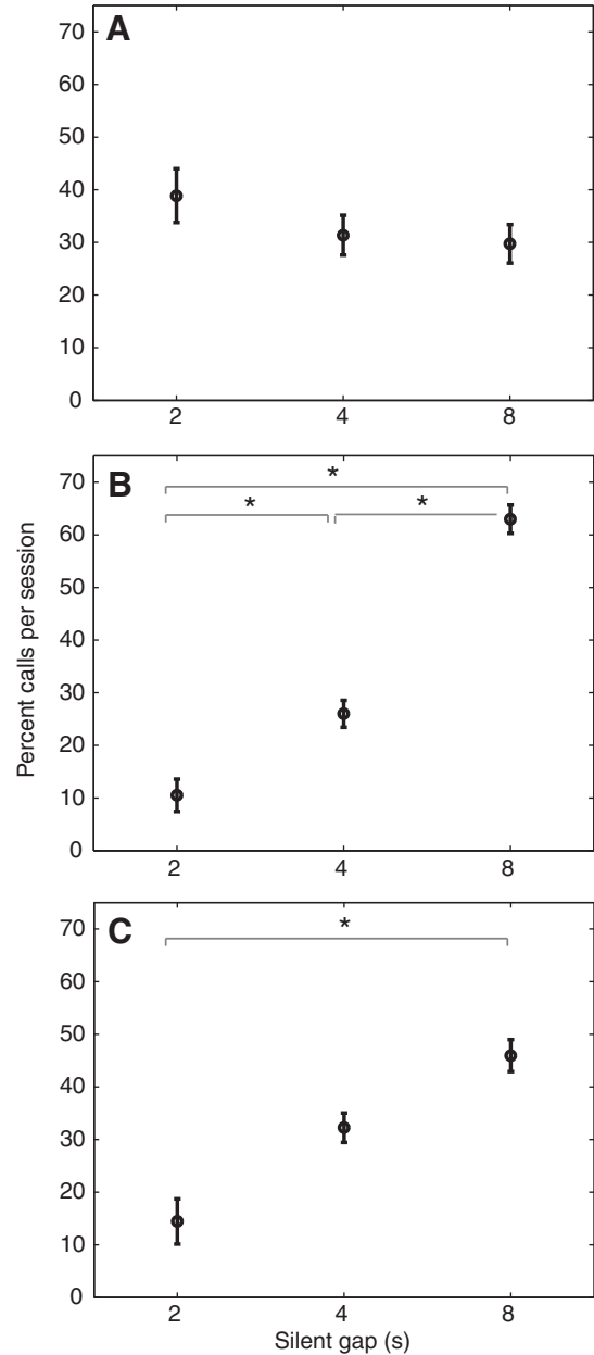
Fig. 2. Percentage of calls initiated per session under the different noise conditions. The majority of calls in the aperiodic conditions were initiated in 4 and 8 s silent gaps. Data shown are means \pm s.e.m. ( N=8 subjects). Statistically significant differences with Bonferroni correction are indicated by an asterisk (* P<0.05 ). (A) Percentage of calls per session during the different periodic noise conditions. (B) Percentage of calls in a given predictable session initiated in 2, 4 or 8 s silent gaps. t -test results: 2 s vs 4 s ( t_7=3.45 , P<0.017 ), 4 s vs 8 s ( t_7=6.87 , P<0.001 ), 2 s vs 8 s ( t_7=9.68 , P<0.001 ). (C) Percentage of calls in a given unpredictable session initiated in 2, 4 or 8 s silent gaps. t -test results: 2 s vs 4 s ( t_7=2.87 , P=0.024 ), 4 s vs 8 s ( t_7=2.57 , P=0.037 ), 2 s vs 8 s ( t_7=4.50 , P<0.017 ).
