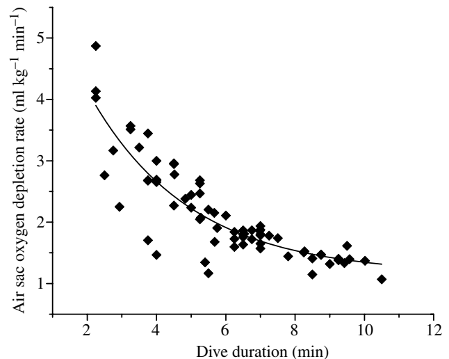
Fig. 10. The estimated air sac O 2 depletion rate based on the previously measured diving respiratory volume of 69 ml kg -1 and the change in air sac O 2 fraction during dives. Regression equation: y = (5.95 \times e^{-x/2.91}) + 1.15 , r^2 = 0.76 , P < 0.0001 .
