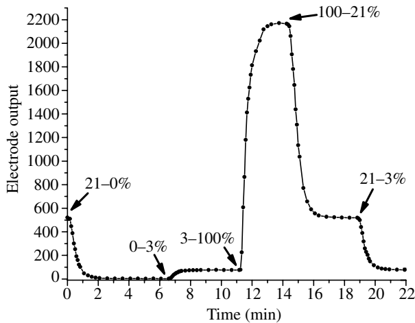
Fig. 1. Response of a P_{O_2} electrode to changes in O_2 concentration. Arrows indicate the time at which the electrode was shifted from one O_2 concentration to another (0, 3, 21, 100% O_2 ).
