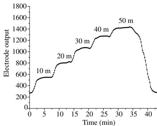
Fig. 3. The output of a P_{O_2} electrode exposed to air in response to step changes in pressure in a recompression chamber. Electrode output, recorded at 15-s intervals, returned to baseline with decompression back to ambient, surface pressure. Equivalent depths (m) are indicated for each step change in pressure.
