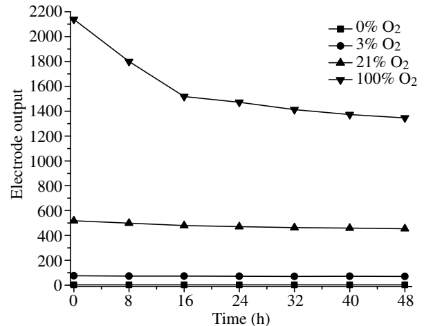
Fig. 2. Drift of a P_{O_2} electrode's output at four different O_2 concentrations over a 48 h calibration.
