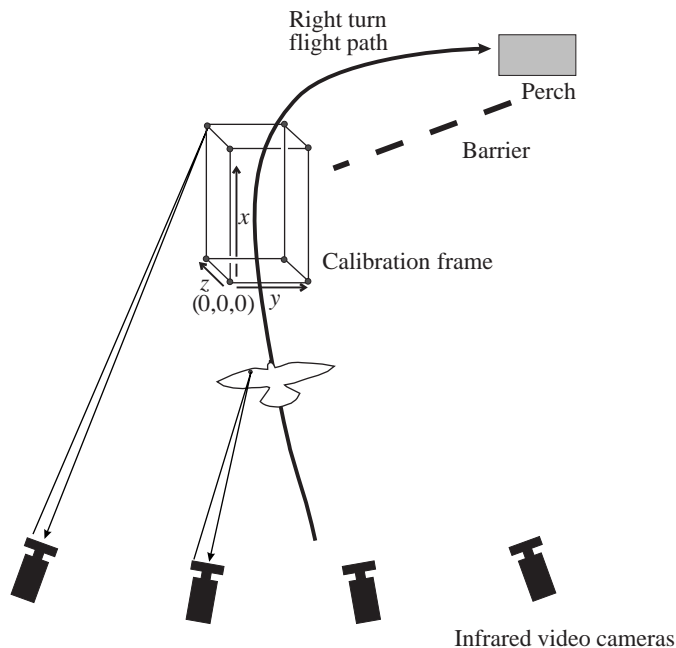
Fig. 1. Recording apparatus, flight path and three-dimensional coordinate ( x, y, z ) space. Maintaining the same height above the floor, the birds performed right or left turns to maneuver around a barrier. The calibration frame was removed after the cameras had been calibrated. The pigeons were in view of the cameras for 2–4 wingbeats at the beginning to intermediate part of the turn (approximately where the calibration frame had been located).
