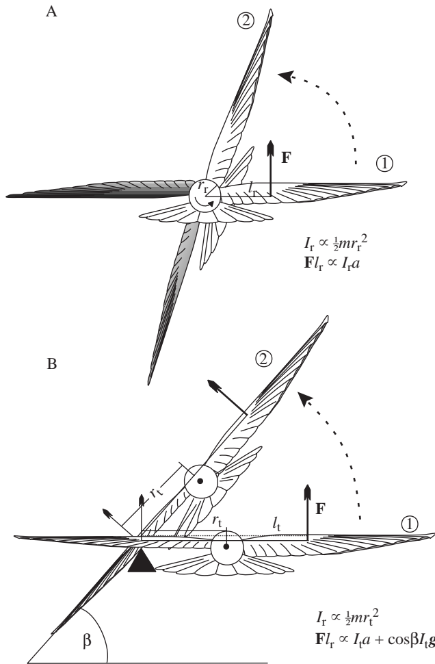
Fig. 16. The moment of inertia ( I ) of a banking bird depends on the method of bank initiation. (A) If weight support lift is not developed on the inside wing (at high speed, this would require, as represented by the shaded inside wing, pronation of the wing to a zero or negative angle of attack or completely folding the wing), the bird will roll around its center of mass ('rotational roll'), which has a relatively low moment of inertia ( I_r \propto \frac{1}{2} m r_r^2 , where m is body mass, a is acceleration, r_r is the radius of gyration around the center of mass with the bird's body modeled as a cylinder). The torque accelerating this inertia would be the lifting force F times the moment arm l_r . (B) If weight-supporting lift (small arrow on left wing) is maintained on the inside wing, it will act as a fulcrum (black triangle) around which the body will move translationally as well as rotationally ('translational roll'). In this case, at any instant during a bank angle ( \beta ) less than 90^\circ , the torque (lifting force F times lever arm l_t ) created by the wing's force asymmetry will not only be accelerating the inertia of the body ( I_t = m r_t^2 times the square of the radius of gyration in translational roll r_t^2 ) but also opposing the inertia's acceleration due to gravity ( g ).
