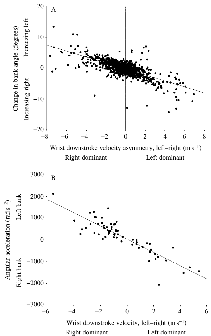
Fig. 7. (A) Relationship between the change in bank angle (i.e. angular velocity) and the wrist downstroke velocity asymmetry immediately preceding it. The correlation indicates the creation of roll following velocity asymmetry. N=969 , \text{ARC}=0.775 , x coefficient= -0.008 , r^2=0.505 , P<0.0001 . (B) Angular acceleration in bank (averaged over approximately 20 ms) versus the asymmetry in wrist velocity immediately preceding it. N=63 , x coefficient= -3.024 , r^2=0.760 , P<0.001 .
