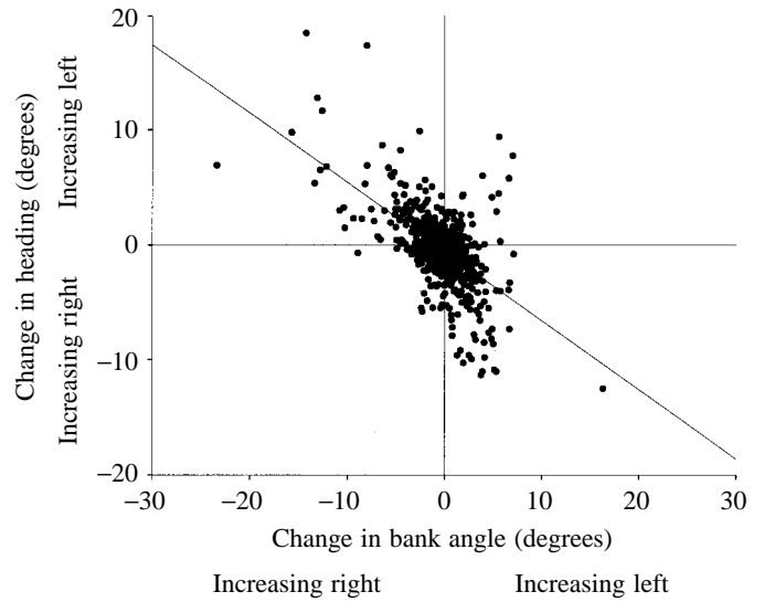
Fig. 5. Relationship between the change in heading and the change in bank angle. The negative correlation indicates the creation of adverse yaw during bank initiation. Data are sequential changes in angle from bank and heading sampled every 5 ms and are thus strongly autocorrelated. Autoregressive models were therefore used: ARC (=autocorrelation coefficient)=0.083, N=2936 , x coefficient=0.375, r^2=0.161 , P<0.00001 .
