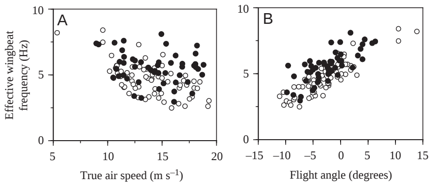
Fig. 3. Effective wingbeat frequency averaged over 20 s with respect to true air speed (A) and flight angle (B). Barn swallows, open circles, N=65 ; house martins, filled circles, N=51 .
