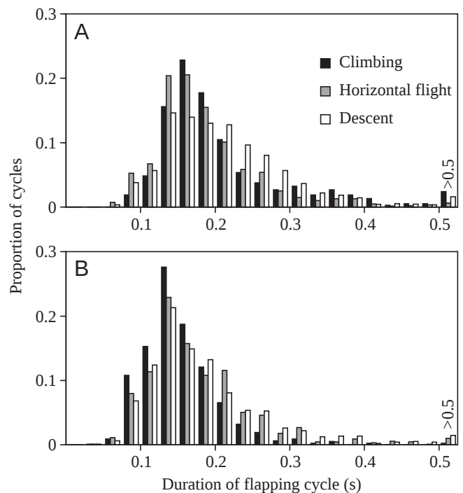
Fig. 2. Relative frequency distribution of the duration of flapping cycles for barn swallows (A) (BS) and house martins (B) (HM) in free flight. Only one 20 s interval per bird was included per flight situation. Climbing (flight angles 3.5 \pm 1.5^\circ ), N_{BS} flapping cycles=372, N_{HM} individuals=6, N_{HM} flapping cycles=779; horizontal flight (flight angles 0 \pm 1.5^\circ ), N_{BS} individuals=13, N_{BS} flapping cycles=1387, N_{HM} individuals=8, N_{HM} flapping cycles=890; descent (flight angles -3.5 \pm 1.5^\circ ), N_{BS} individuals=18, N_{BS} flapping cycles=1691, N_{HM} individuals=9, N_{HM} flapping cycles=952. True air speed was restricted to 10–16 m s -1 .
