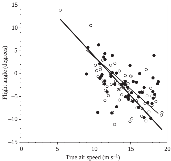
Fig. 4. Flight angle with respect to true air speed for barn swallows (open symbols, N=65 ) and house martins (filled symbols, N=51 ). The geometric mean regressions for barn swallows (thin line) and house martins (bold line) are shown. The correlation between air speed and flight angle is much higher for barn swallows ( r=-0.71 ) than for house martins ( r=-0.44 ) even when the two highest values of flight angle for barn swallows are excluded.
