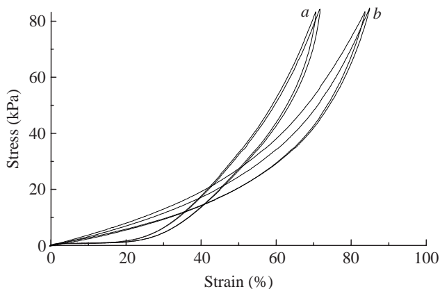
Fig. 6. The effect of treatment with guanidine hydrochloride on the stress-strain behaviour of a sample of zonule (curve a ) in PBS and (curve b ) in TBS+EGTA. Two stress-strain cycles are shown for each treatment. Subsequent bathing in high [Ca^{2+}]TBS reverts the behaviour to that in curve ( a ). The effects of addition/removal of Ca^{2+} are reversible.
