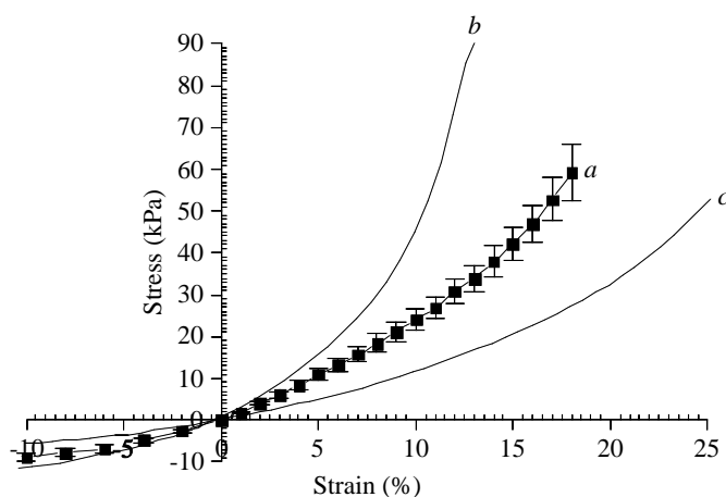
Fig. 4. Curve a is the mean stress-strain curve calculated from the load-elongation data for 11 samples. Values are means \pm S.E.M. Curve b is the stress-strain curve for the least compliant sample. Curve c is the stress-strain curve for the most compliant sample.
