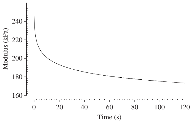
Fig. 8. Stress-relaxation behaviour of a zonular filament sample. Relaxation modulus (stress/strain) versus time for a specimen held at fixed extension after extension at 20 \text{ mm min}^{-1} to a load of 1 g.
