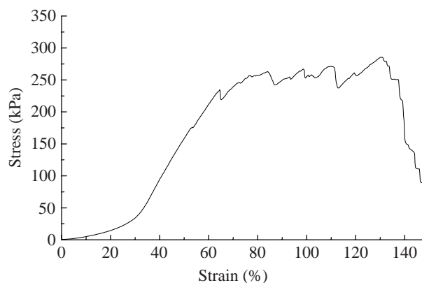
Fig. 7. Stress-strain curve for a zonular filament sample strained to failure.
