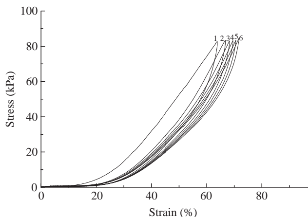
Fig. 3. Stress-strain diagram showing pre-conditioning cycles 1-6 for a typical specimen.
