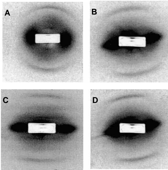
Fig. 1. Small-angle X-ray diffraction patterns from two specimens (A,B) showing different degrees of structural ordering at initial length. Extension by approximately 50% of the specimen in A results in increased ordering (C), but similar extension of the specimen in B results in little change (D).
