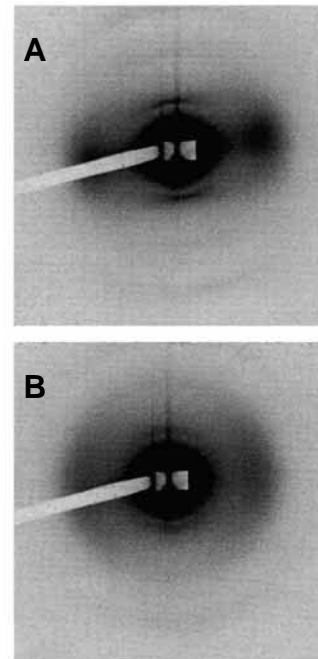
Fig. 2. Microfocus (100 \mu\text{m} spot size) small-angle X-ray diffraction patterns from two different areas (A,B) on the same zonular filament preparation at rest length. (A) Relatively ordered/strained area; (B) less well-ordered area.
